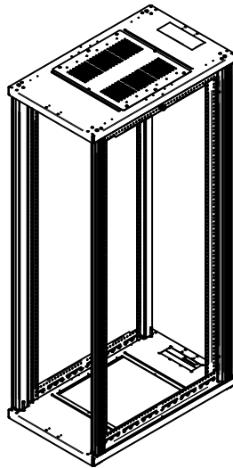
F/D1000
